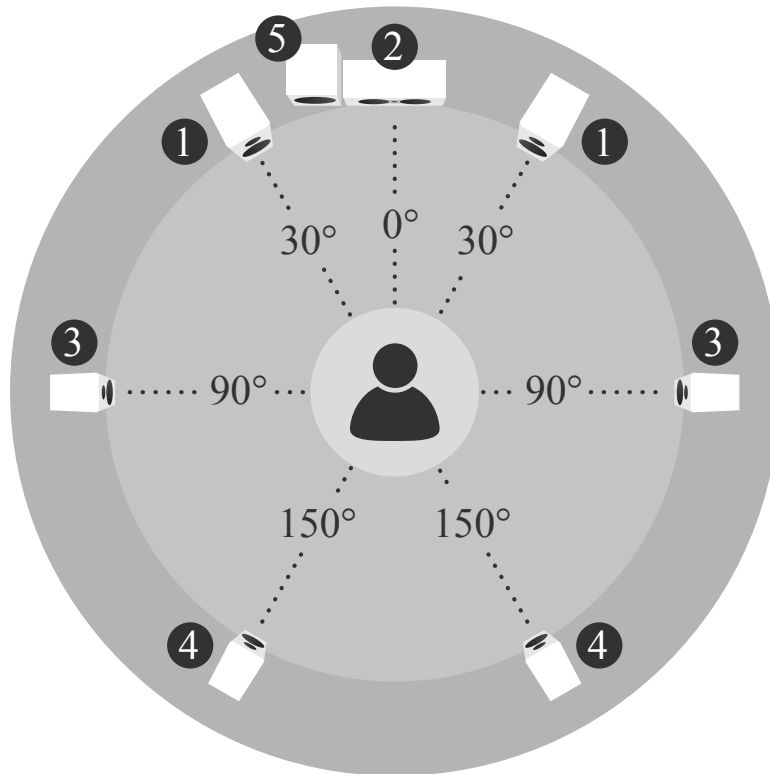
Figure 6: 5.1 and 7.1 multi-channel loudspeaker setup
